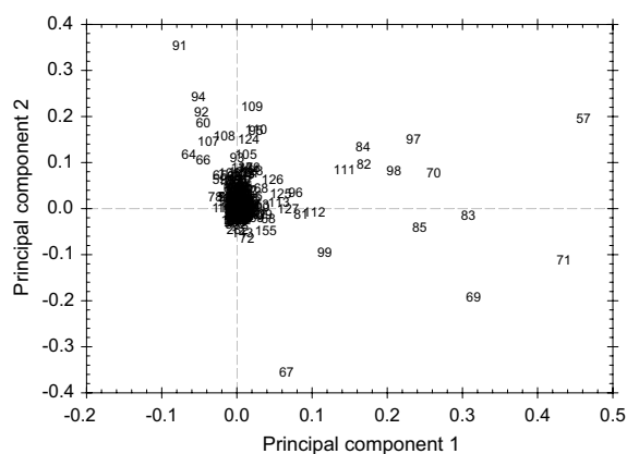
Fig. 8 Principal components analysis loadings for spectral range m/z = 57 –450 of whole-soil and isolated fraction samples combined. Numerical symbols represent individual m/z values
