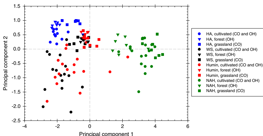
Fig. 7 Principal components analysis scores for spectral range m/z = 57 –450 of whole-soil and isolated fraction samples combined. Black symbols are whole-soil samples, blue symbols are humic acid samples, red symbols are humin samples and green symbols are non-acid hydrolysable samples. ●, cultivated samples (CO and OH); ▼, forest samples (OH); ■, grassland samples (CO)
