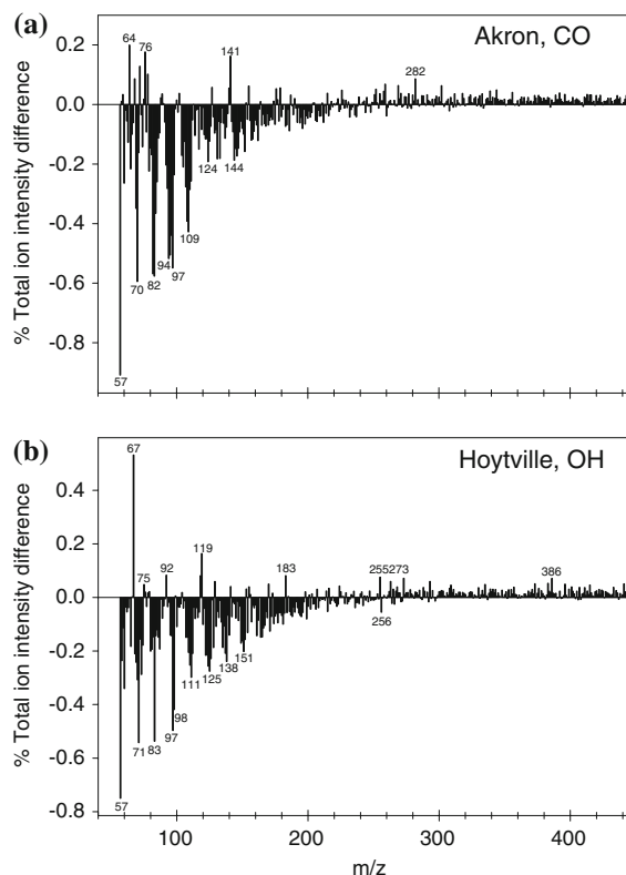
Fig. 3 Difference spectra of cultivated minus native whole-soil samples of the normalized mass spectra for spectral range m/z = 57 –450 for (a) Akron, CO, and (b) Hoytville, OH
